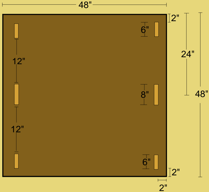
PLAN VIEW
