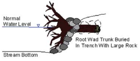
Section View
