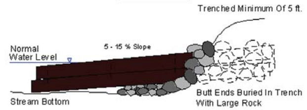
Section View
