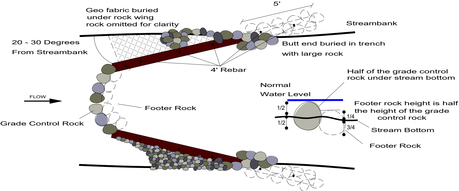
Section View
