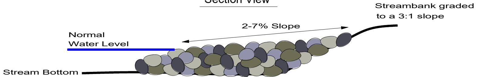
Section View
