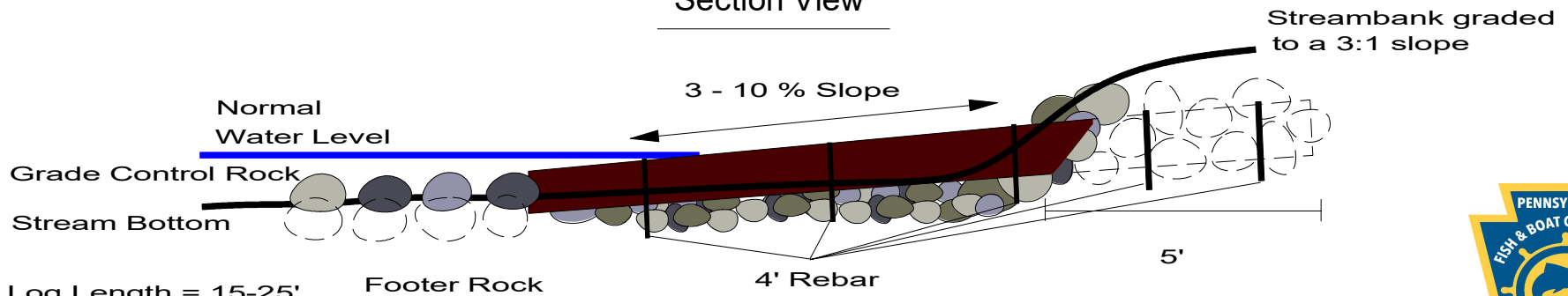
Section View
