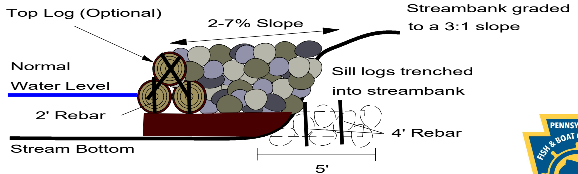
Section View
