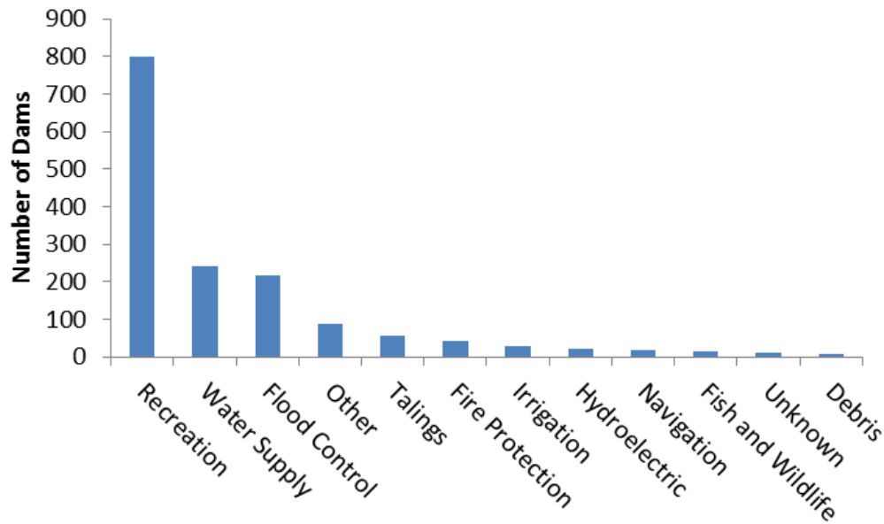
Fig. 3.18. Primary purpose of Pennsylvania dams identified in the U.S. Army Corps of Engineers, National Inventory of Dams (NID).
