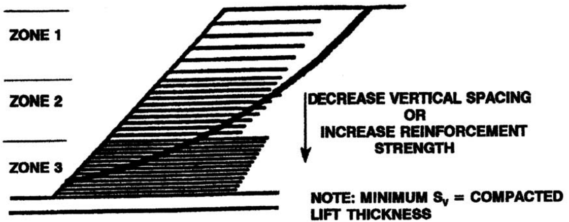
A) SPACING VERSUS REINFORCEMENT STRENGTH
