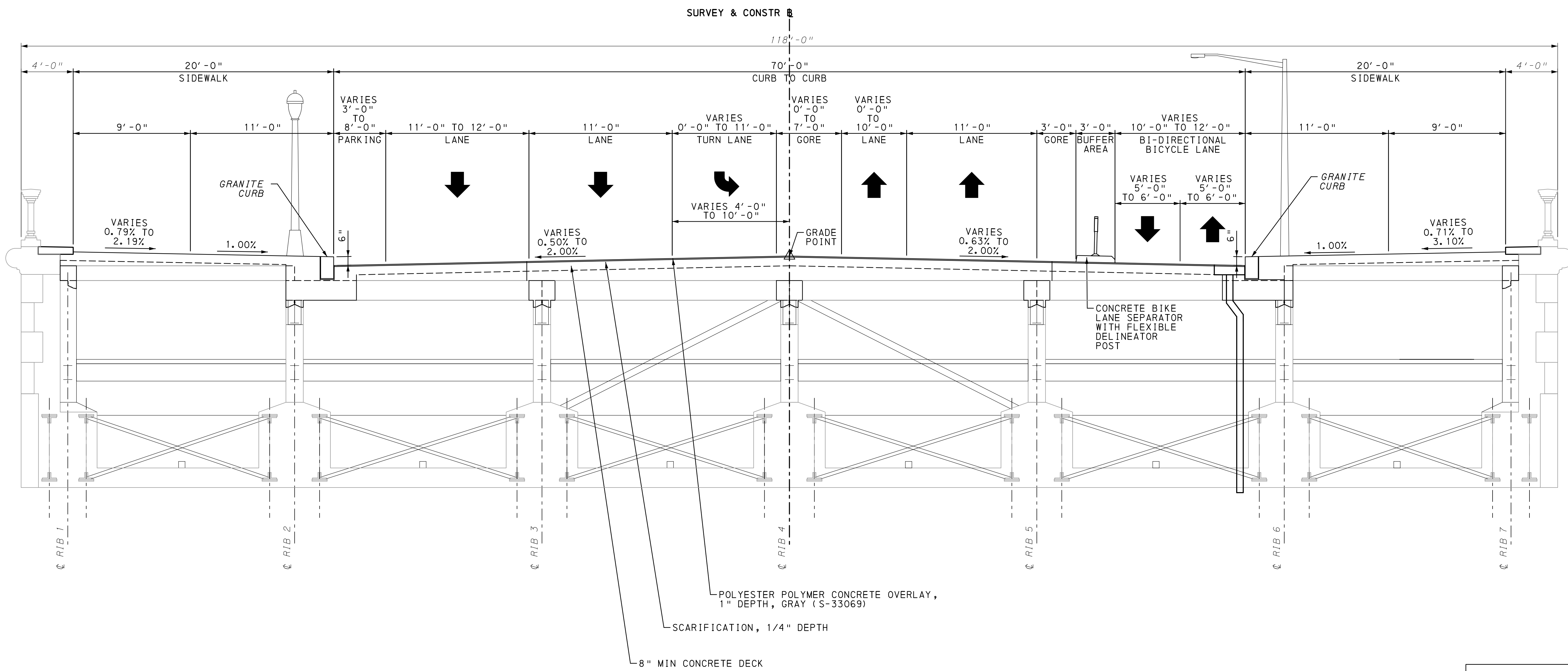
MARKET STREET OVER SCHUYLKILL RIVER LOOKING EAST NOT TO SCALE
