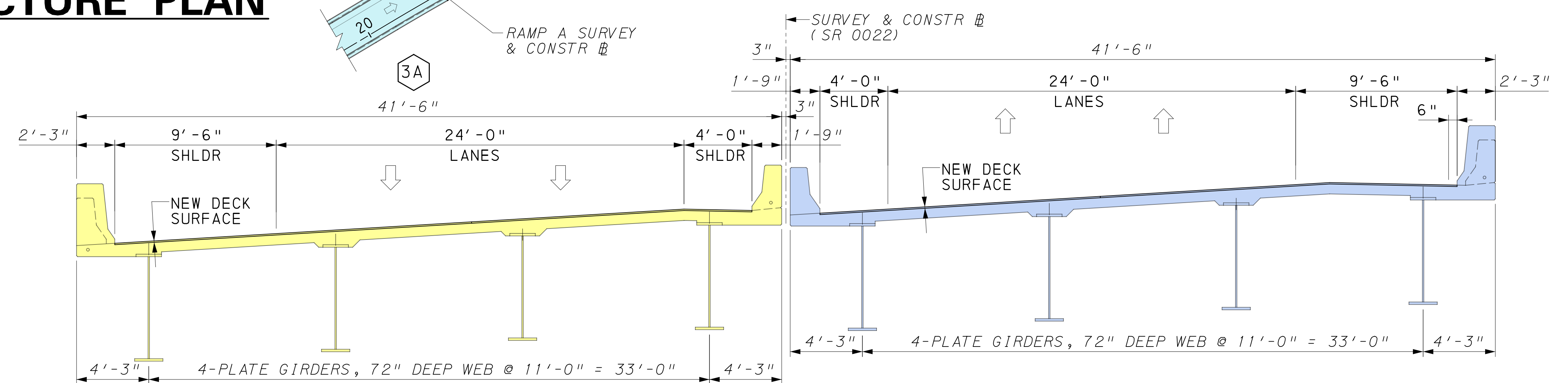
TYPICAL SECTION
