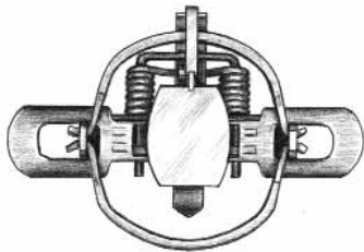
Figure EC5a. Unmodified jaw coil-spring trap (open)
