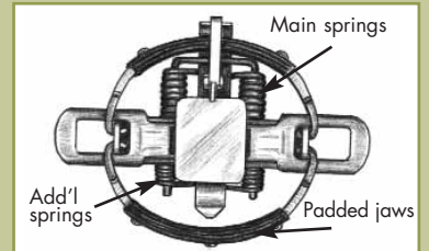
Figure EC4a. Padded jaw coil-spring trap (open)
